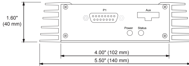
FIGURE 17. VBL2350 front view and dimensions
