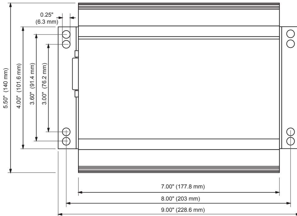
FIGURE 18. VBL2350 top view and dimensions
