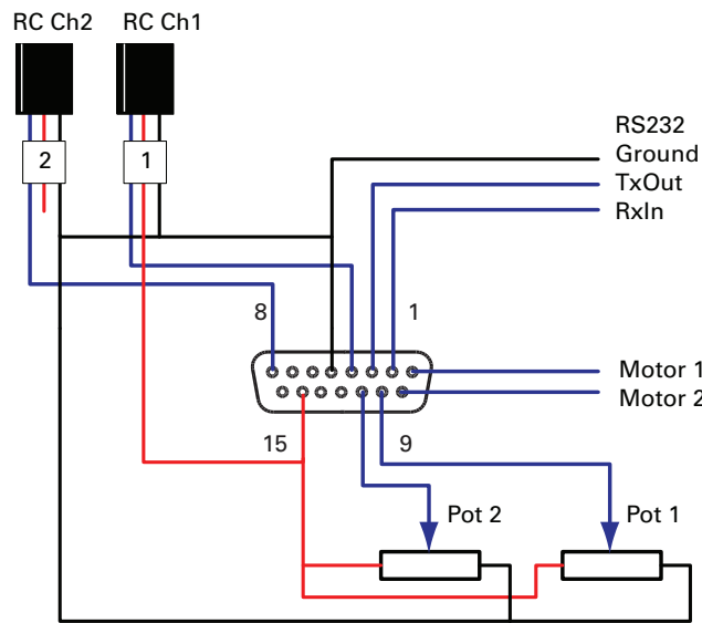
FIGURE 14. Factory default pins assignment
